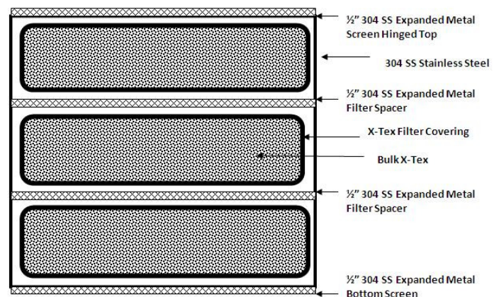
Waterway Solutions' Multi-Stage Hanging Filter Box with X-Tex Hydrocarbon Filters
